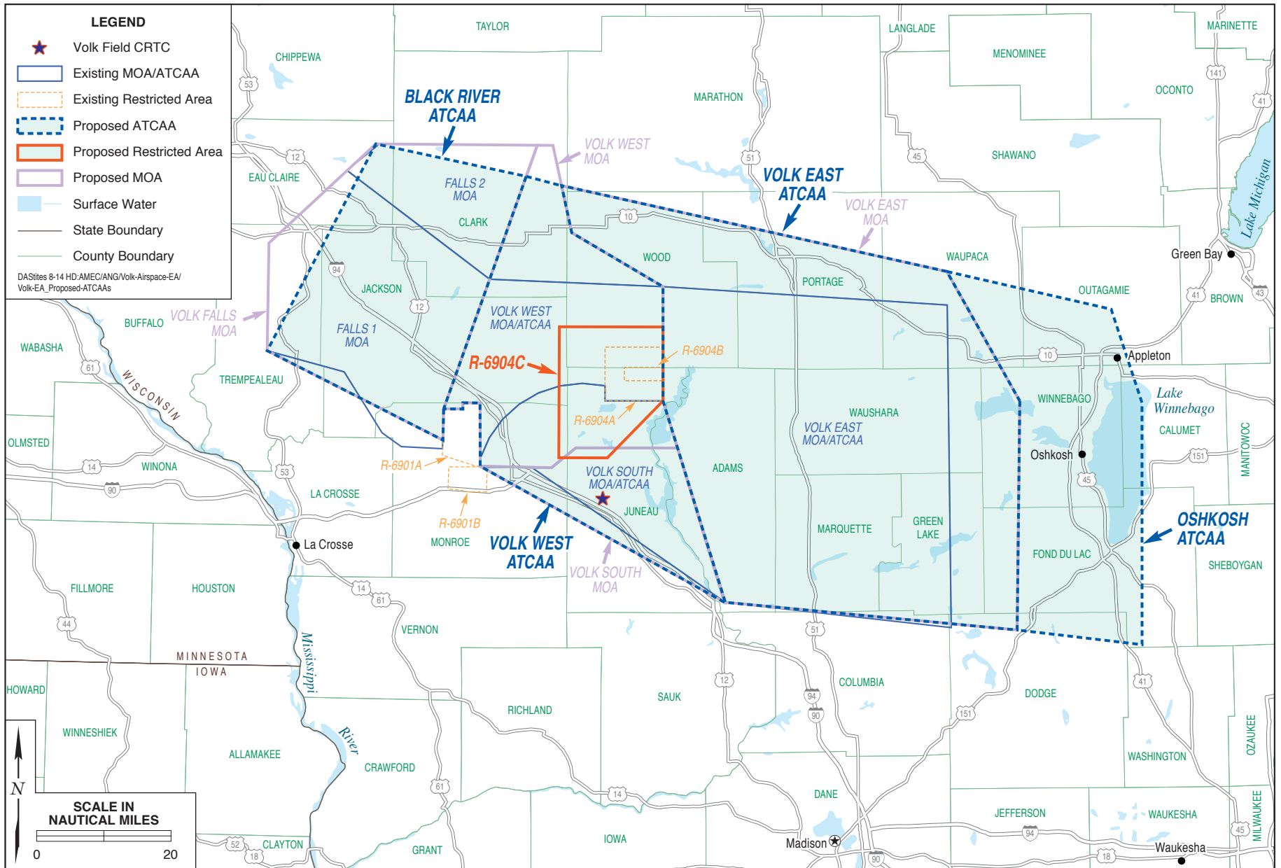
Proposed Air Traffic Control Assigned Airspace and Restricted Area
